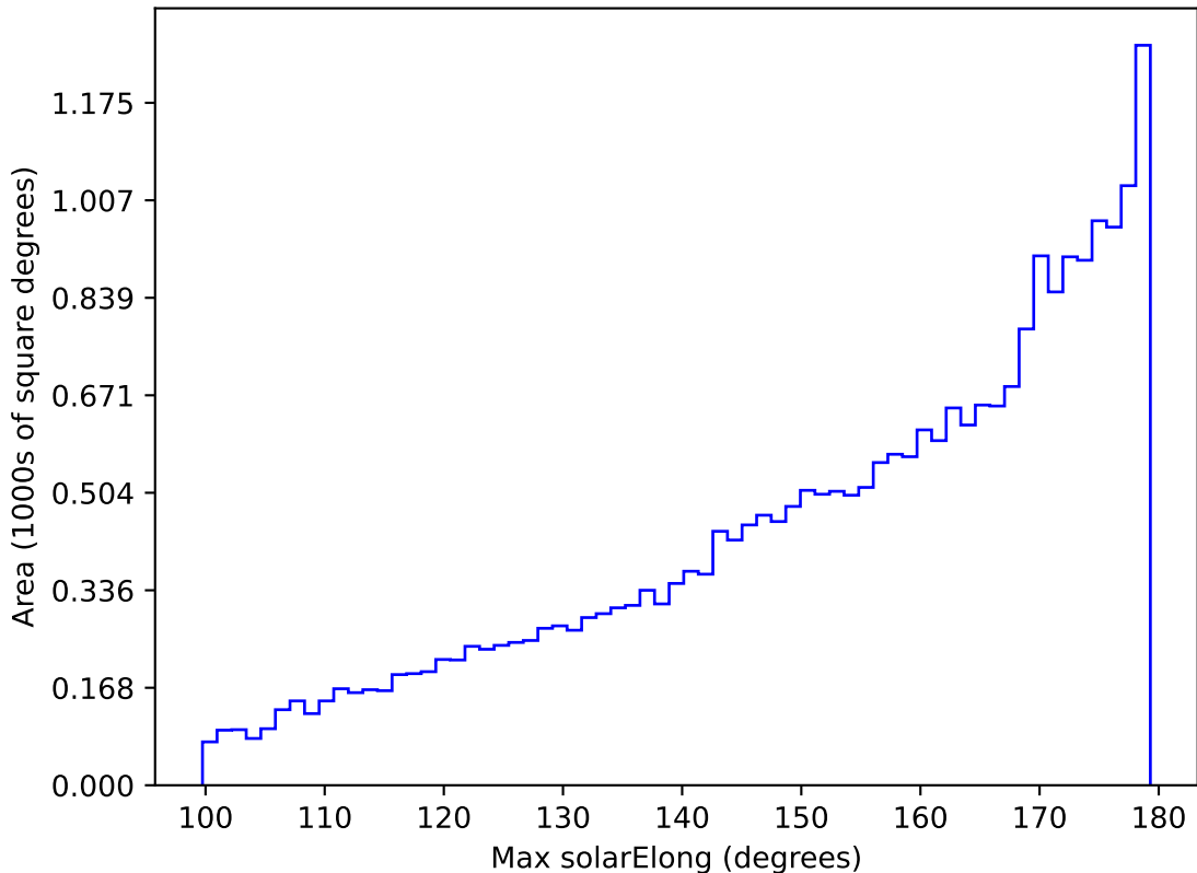
ddf_acor_sf10_lsf30_lsr10_v3.4_10yrs All sky i band: Max solarElong
