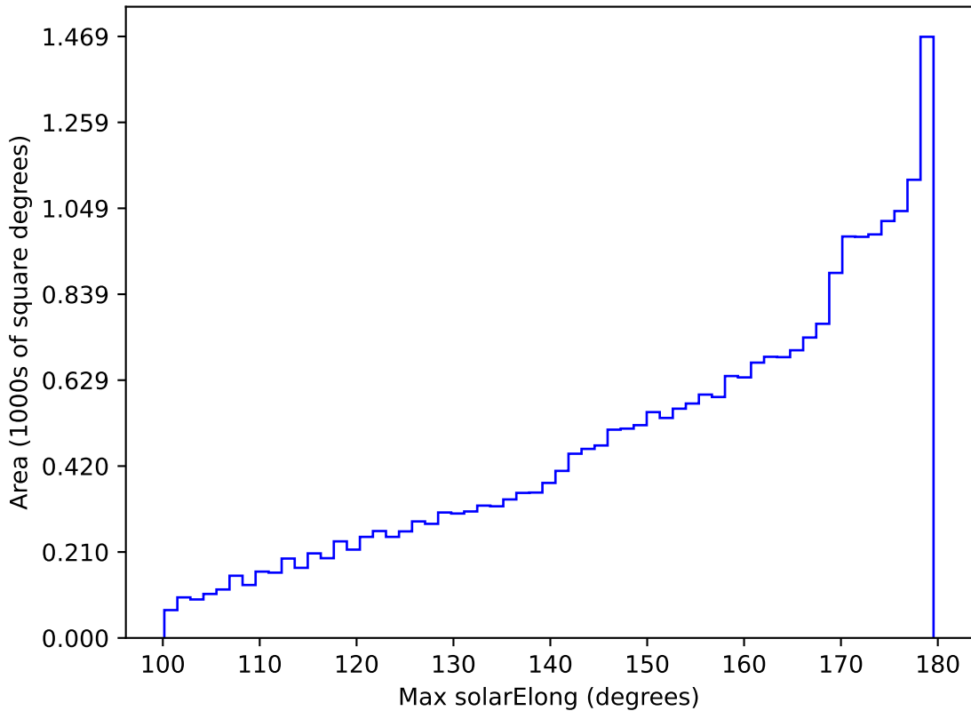
ddf_acor_sf10_ls30_lsr10_v3.4_10yrs All sky all bands: Max solarElong
