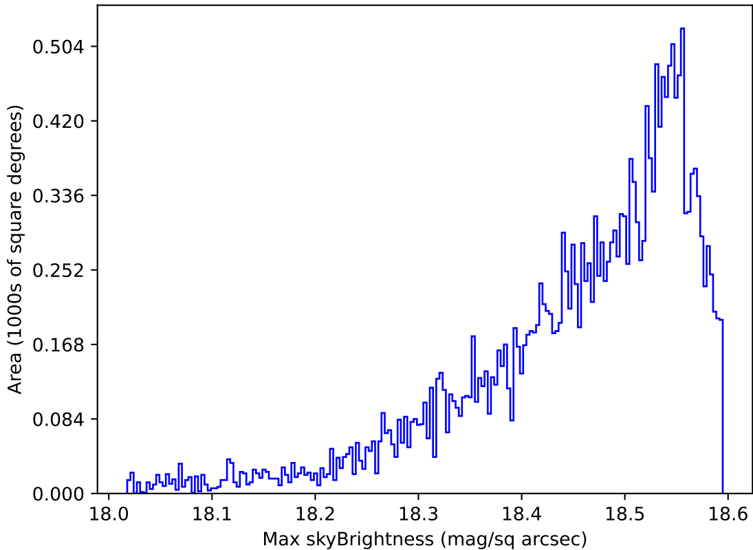
ddf_acor_sf10_lsf30_lsr10_v3.4_10yrs Yr 1 y band: Max skyBrightness
