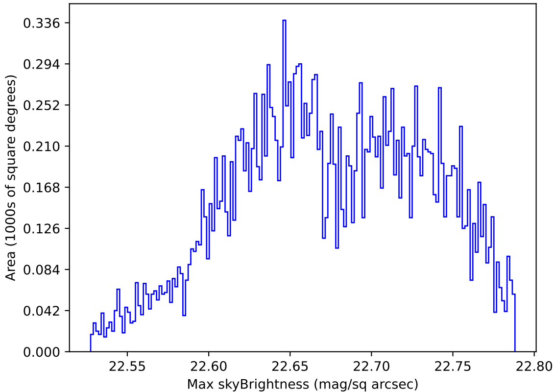
ddf_acor_sf10_lsf30_lsr10_v3.4_10yrs Yr 1 u band: Max skyBrightness
