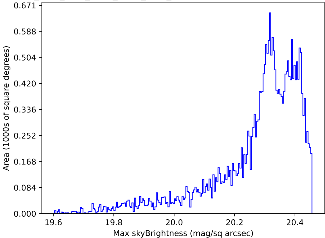
ddf_acor_sf10_lsf30_lsr10_v3.4_10yrs Yr 1 i band: Max skyBrightness
