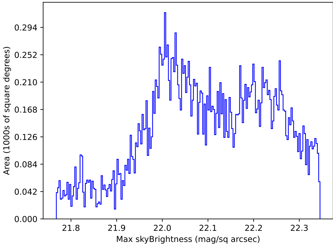
ddf_acor_sf10_ls30_lsr10_v3.4_10yrs Yr 1 g band: Max skyBrightness
