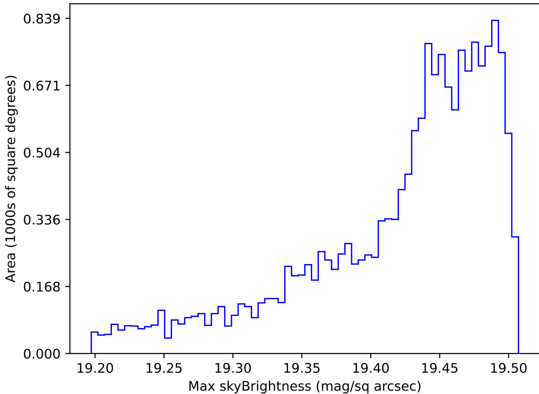
ddf_acor_sf10_lsf30_lsr10_v3.4_10yrs WFD z band: Max skyBrightness
