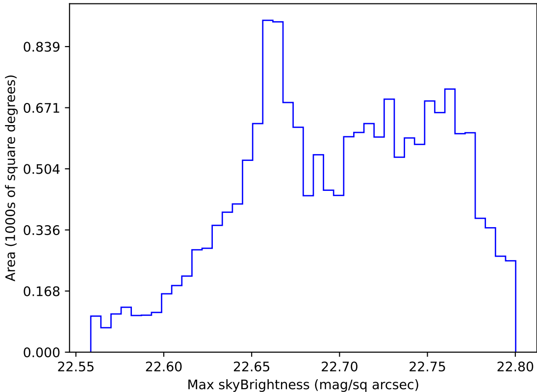
ddf_acor_sf10_lsf30_lsr10_v3.4_10yrs WFD u band: Max skyBrightness
