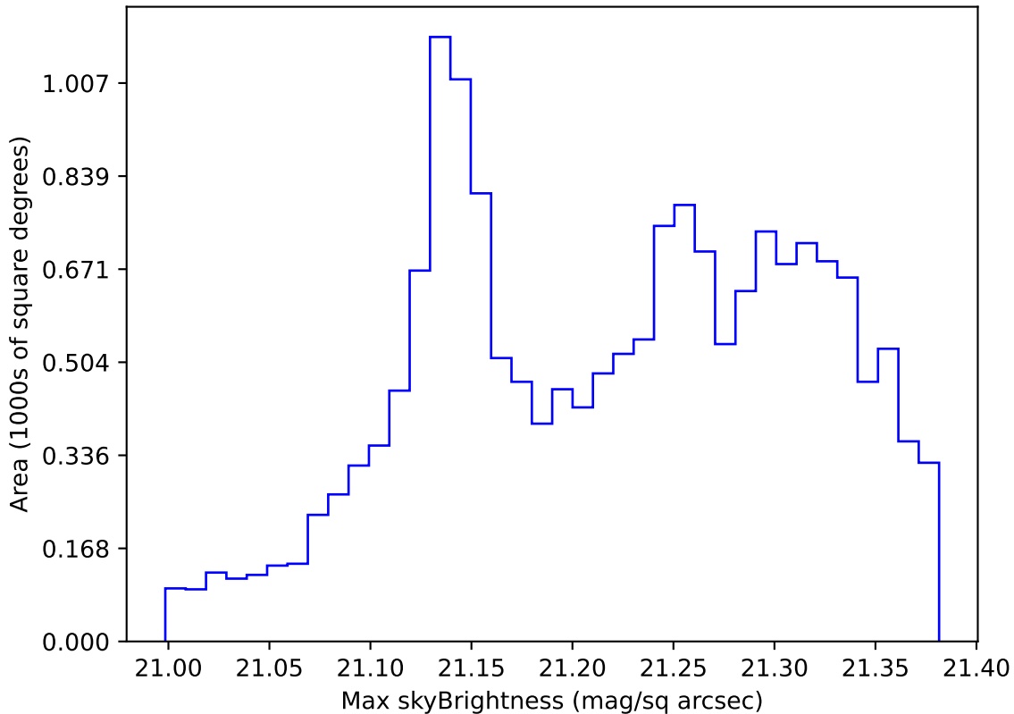
ddf_acor_sf10_lsf30_lsr10_v3.4_10yrs WFD r band: Max skyBrightness
