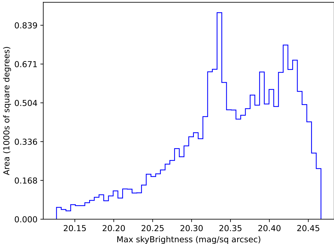
ddf_acor_sf10_lsf30_lsr10_v3.4_10yrs WFD i band: Max skyBrightness
