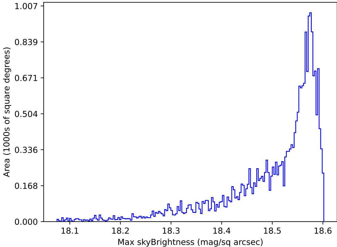
ddf_acor_sf10_lsf30_lsr10_v3.4_10yrs All sky y band: Max skyBrightness
