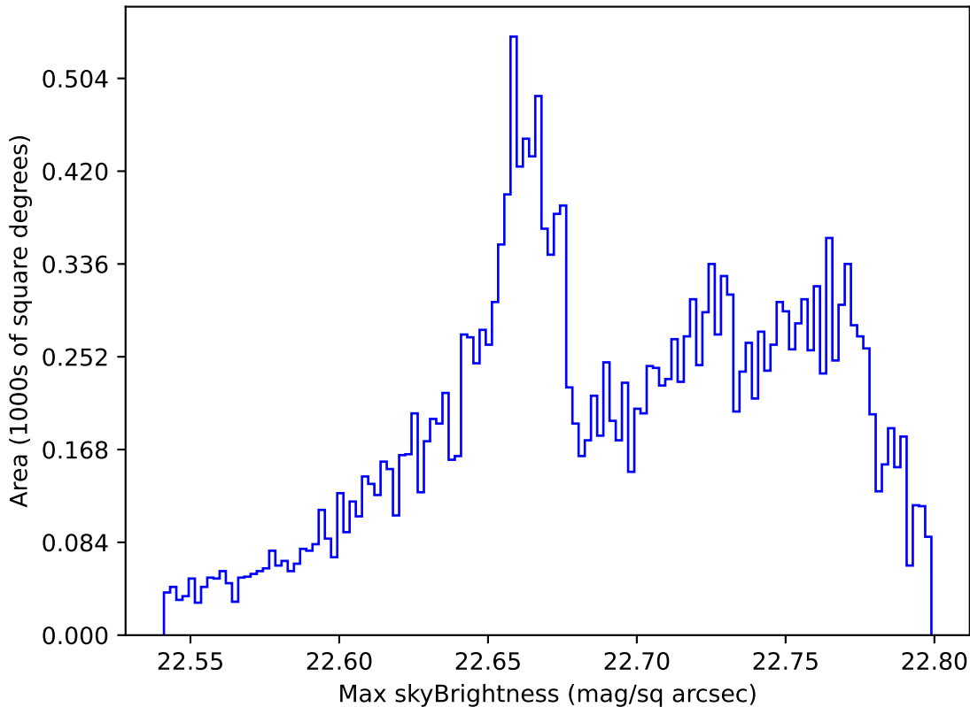
ddf_acor_sf10_lsf30_lsr10_v3.4_10yrs All sky u band: Max skyBrightness
