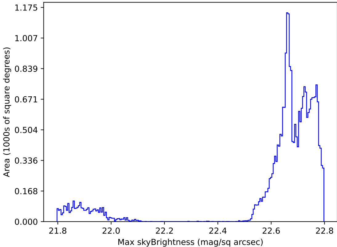
ddf_acor_sf10_ls30_lsr10_v3.4_10yrs All sky all bands: Max skyBrightness
