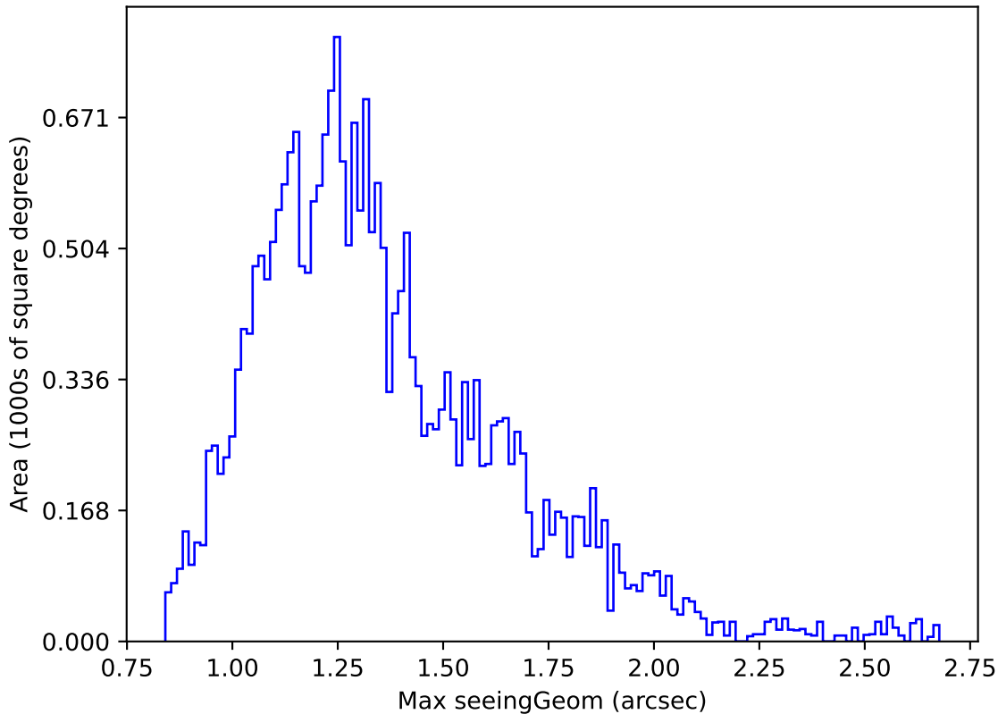
ddf_acor_sf10_lsf30_lsr10_v3.4_10yrs Yr 1 r band: Max seeingGeom
