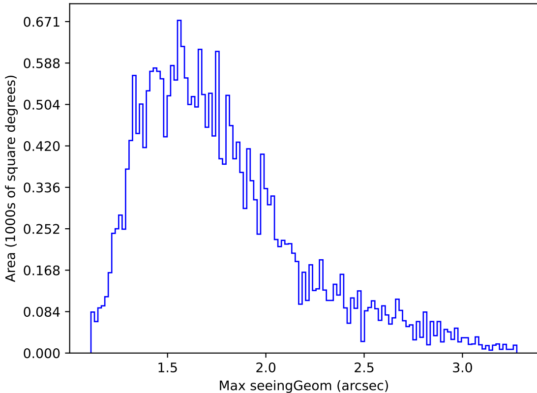
ddf_acor_sf10_lsf30_lsr10_v3.4_10yrs Yr 1 all bands: Max seeingGeom
