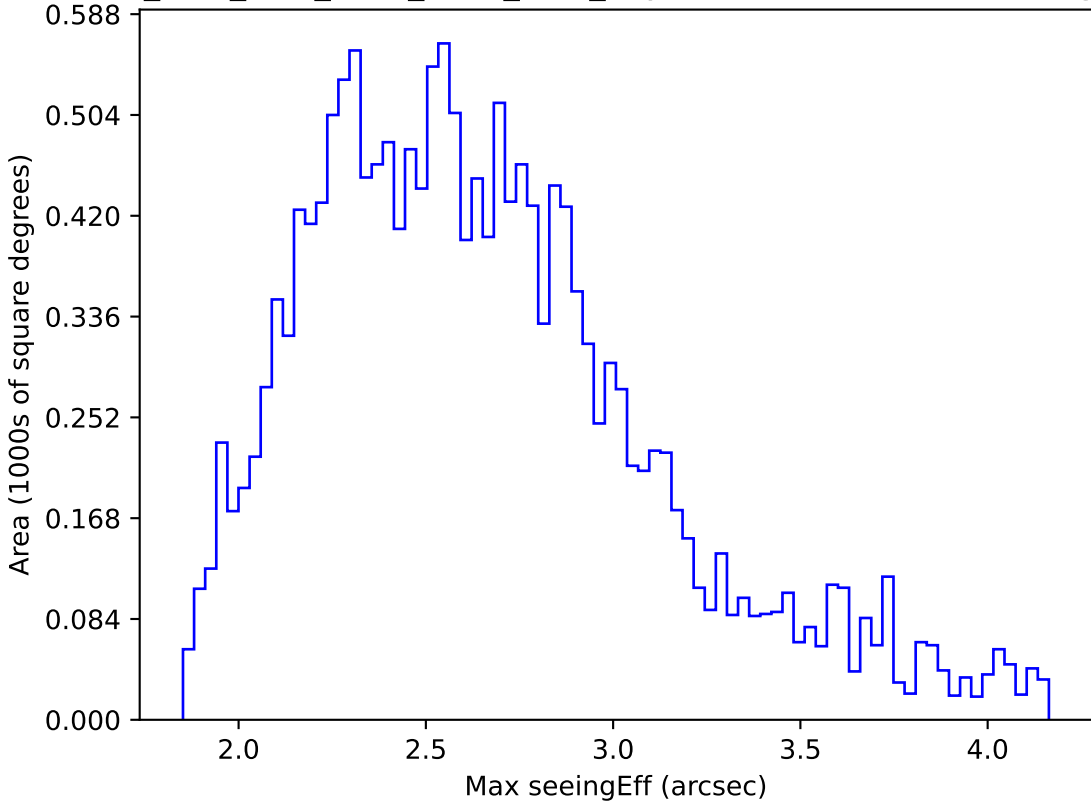
ddf_acor_sf10_lsf30_lsr10_v3.4_10yrs WFD r band: Max seeingEff
