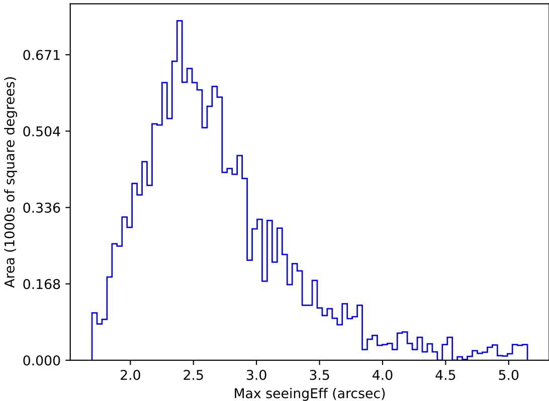
ddf_acor_sf10_lsf30_lsr10_v3.4_10yrs WFD i band: Max seeingEff
