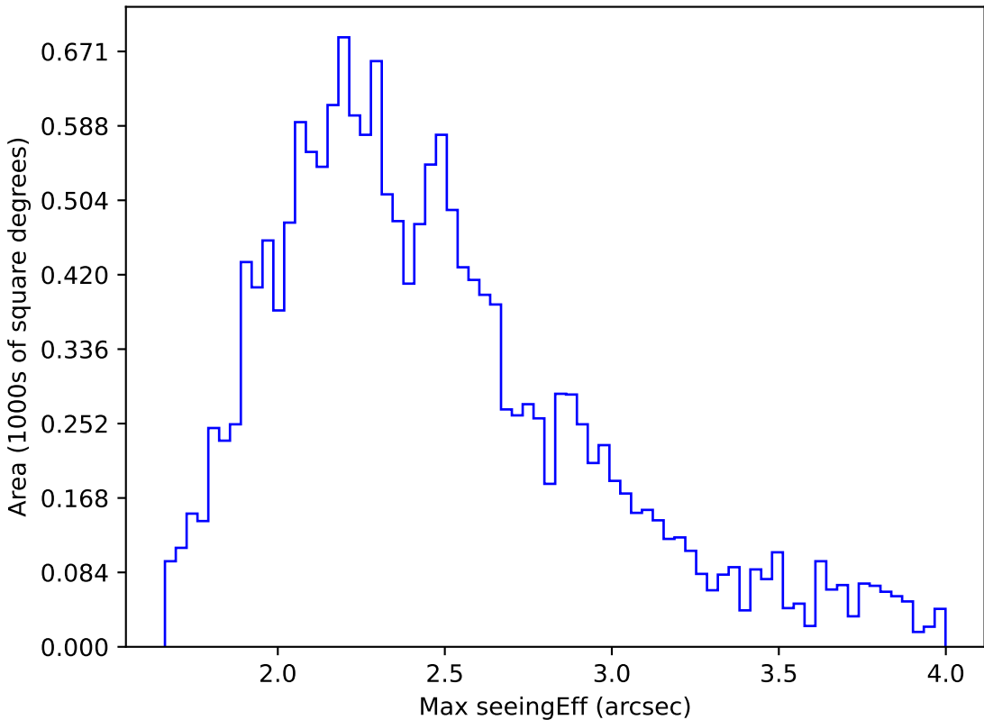
ddf_acor_sf10_lsf30_lsr10_v3.4_10yrs WFD g band: Max seeingEff
