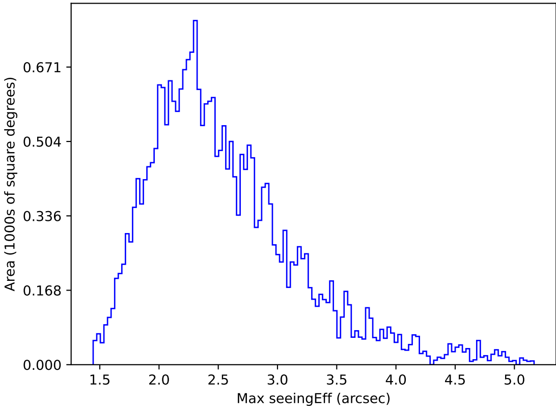
ddf_acor_sf10_lsf30_lsr10_v3.4_10yrs All sky z band: Max seeingEff
