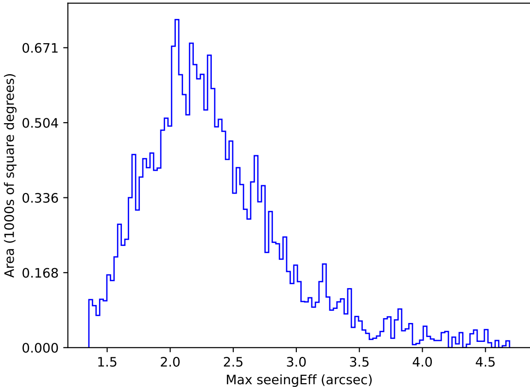
ddf_acor_sf10_ls30_lsr10_v3.4_10yrs All sky y band: Max seeingEff
