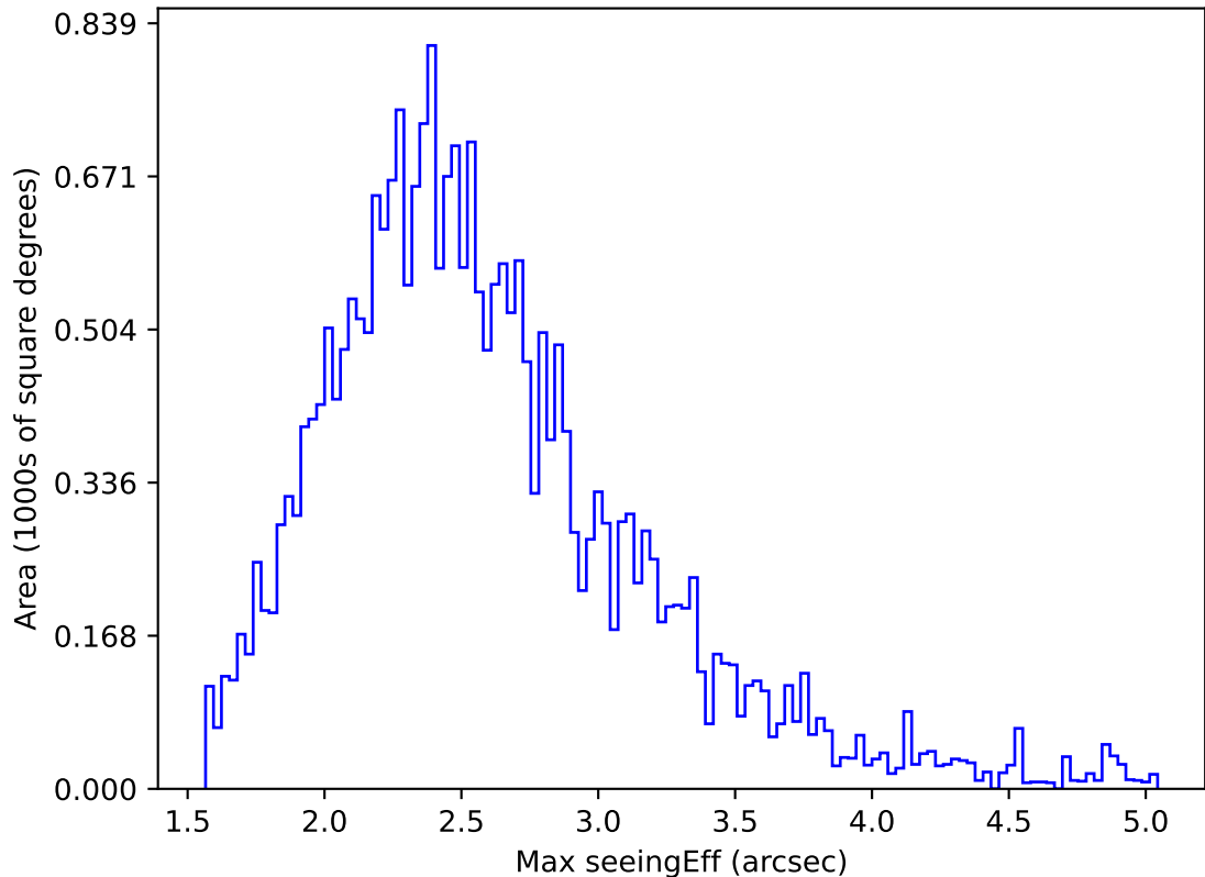
ddf_acor_sf10_lsf30_lsr10_v3.4_10yrs All sky i band: Max seeingEff
