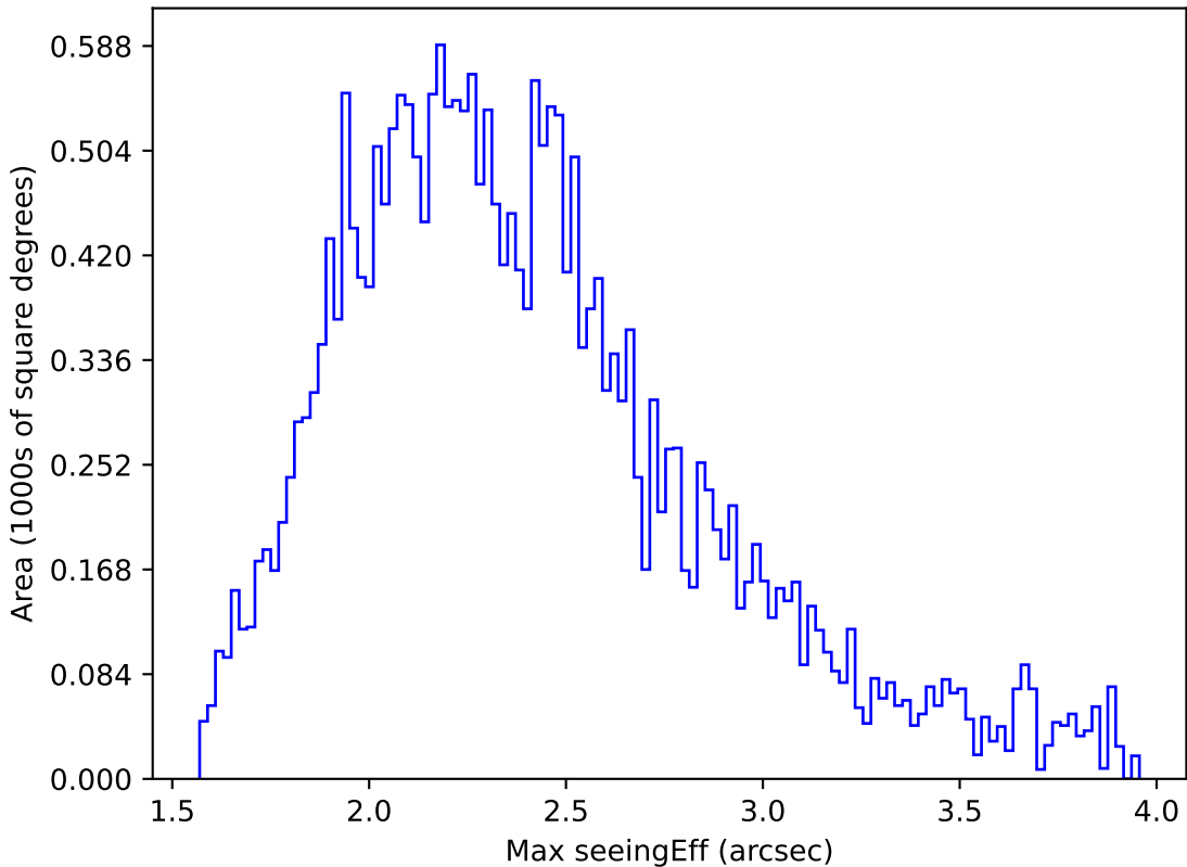
ddf_acor_sf10_lsf30_lsr10_v3.4_10yrs All sky g band: Max seeingEff
