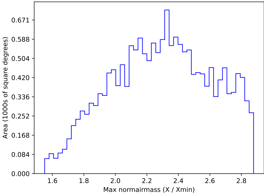
ddf_acor_sf10_lsf30_lsr10_v3.4_10yrs WFD i band: Max normairmass
