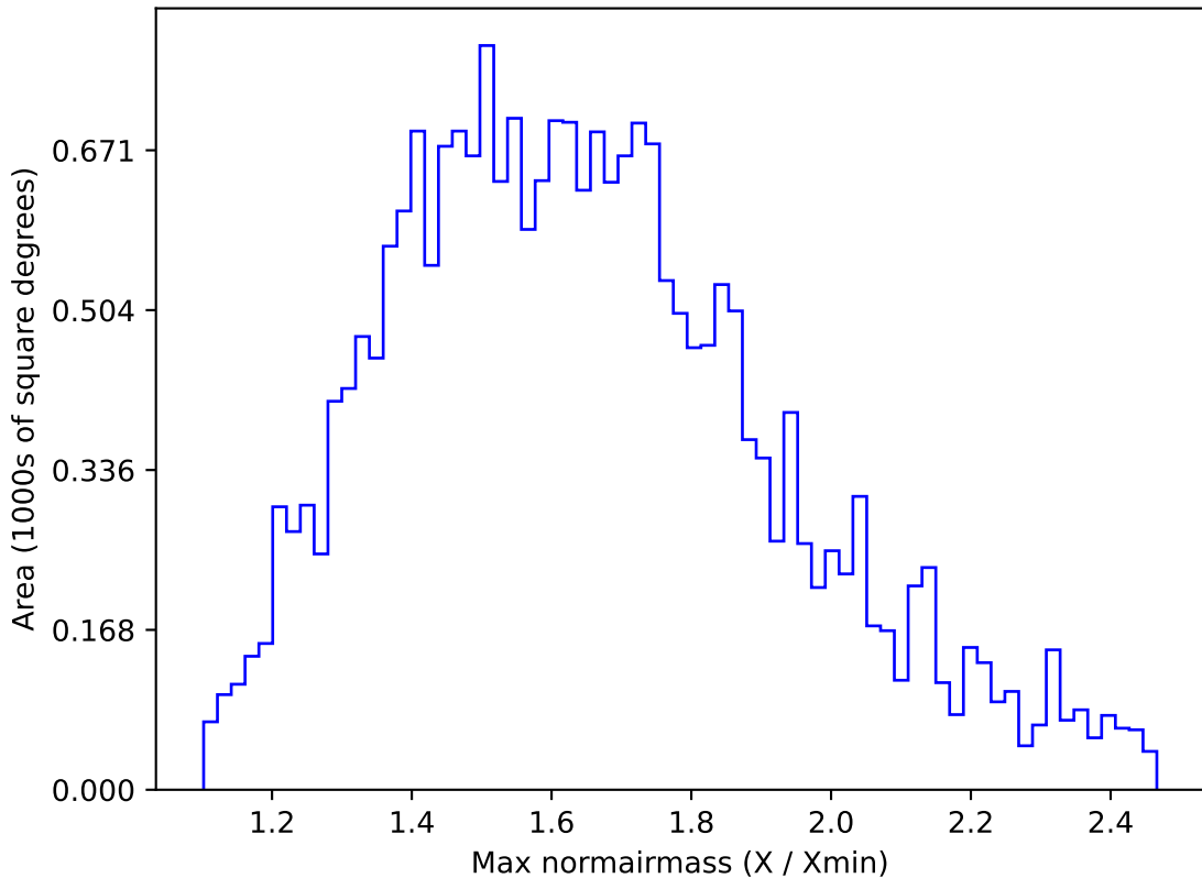
ddf_acor_sf10_lsf30_lsr10_v3.4_10yrs All sky u band: Max normairmass
