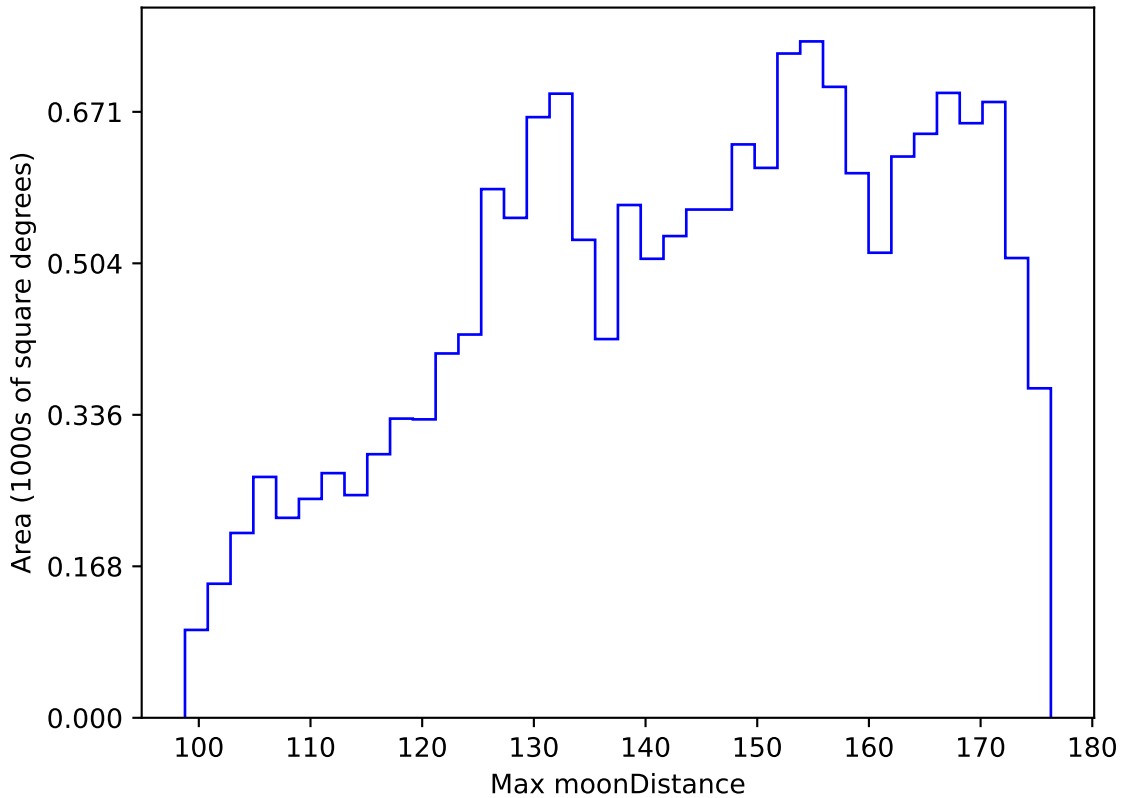
ddf_acor_sf10_lsf30_lsr10_v3.4_10yrs WFD y band: Max moonDistance
