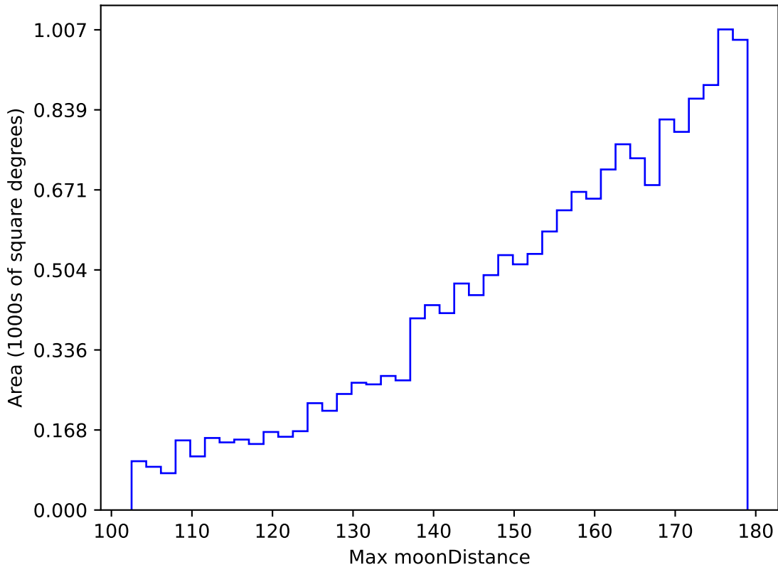
ddf_acor_sf10_lsf30_lsr10_v3.4_10yrs WFD u band: Max moonDistance
