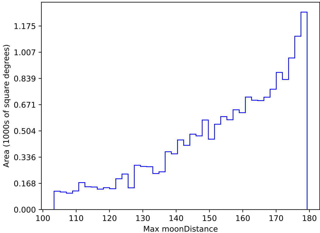
ddf_acor_sf10_lsf30_lsr10_v3.4_10yrs WFD i band: Max moonDistance
