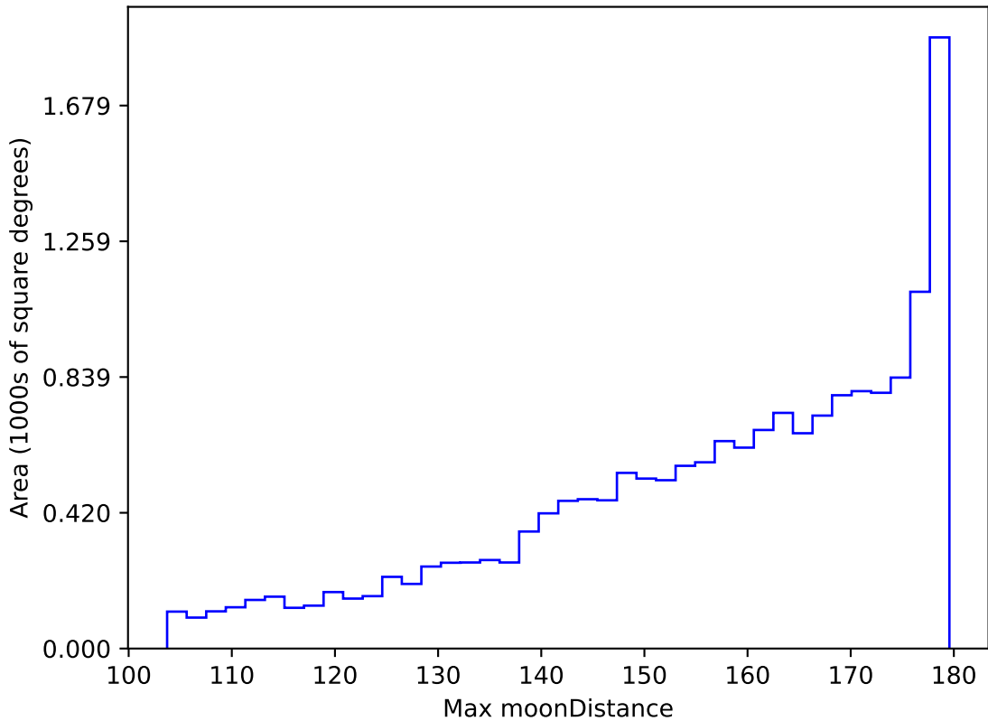
ddf_acor_sf10_lsf30_lsr10_v3.4_10yrs WFD all bands: Max moonDistance
