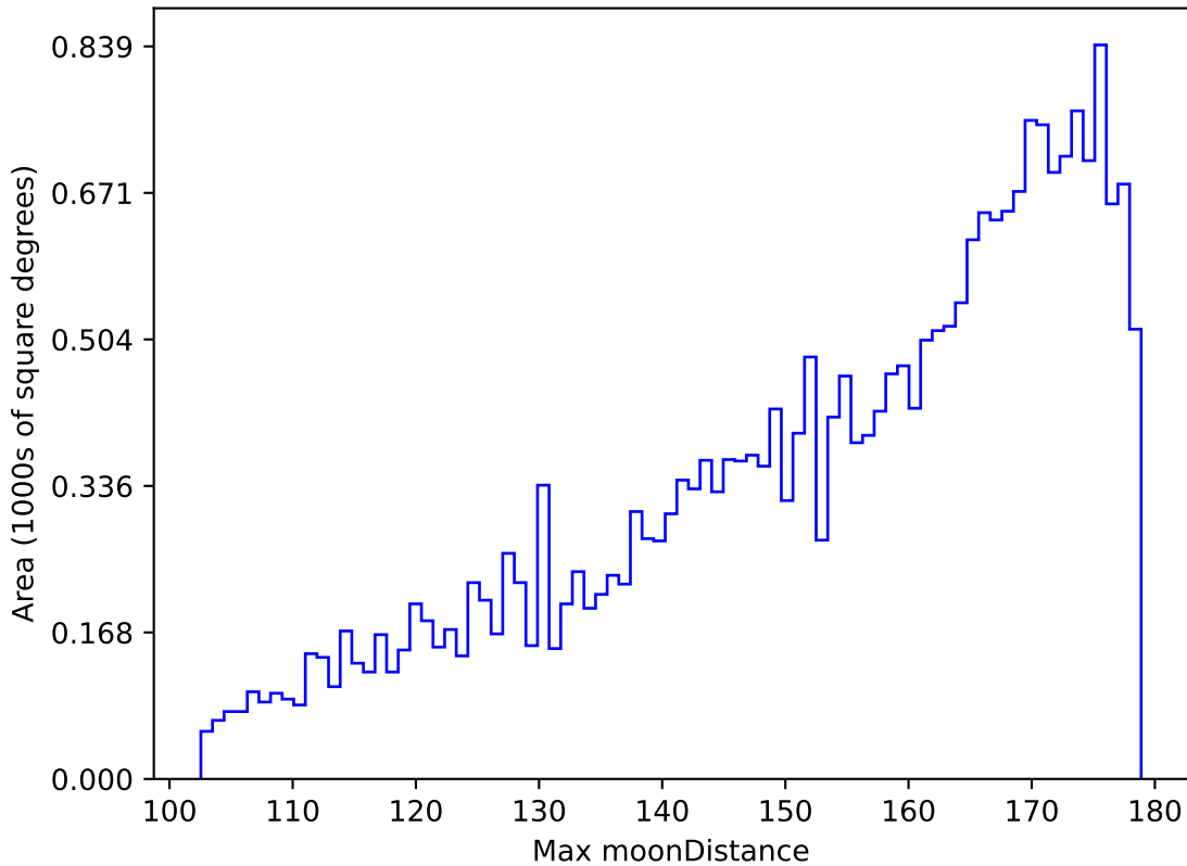
ddf_acor_sf10_lsf30_lsr10_v3.4_10yrs All sky z band: Max moonDistance
