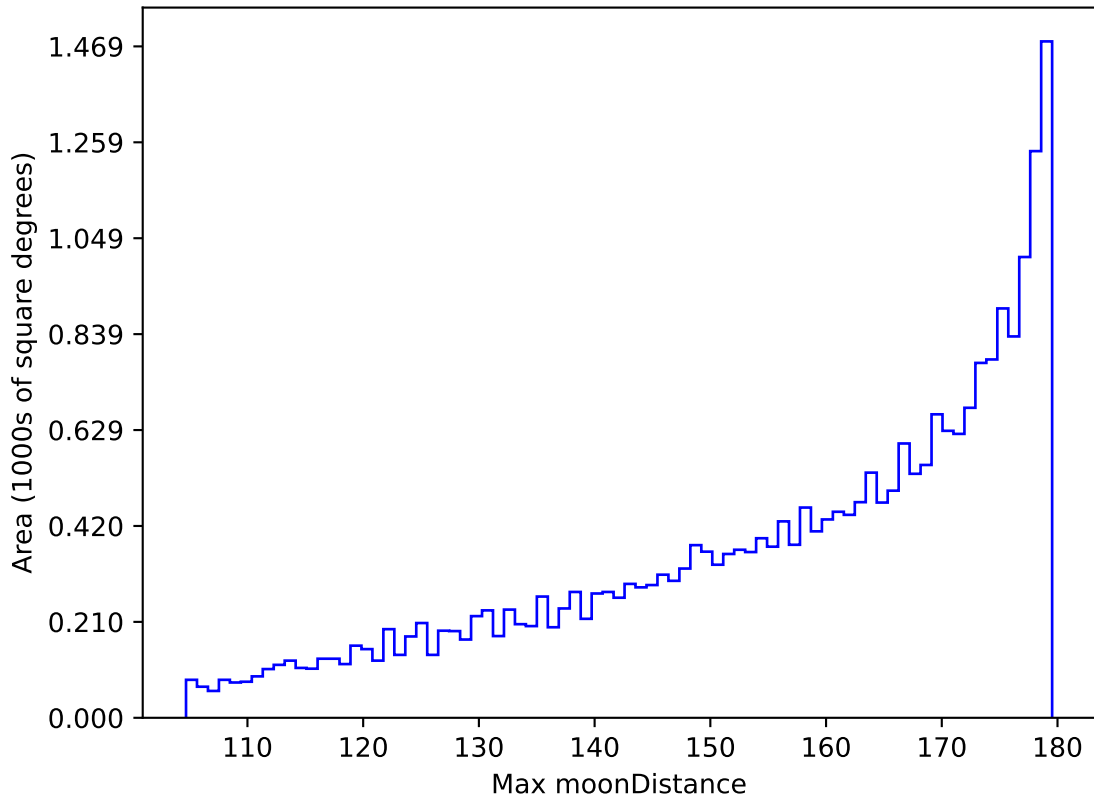
ddf_acor_sf10_lsf30_lsr10_v3.4_10yrs All sky all bands: Max moonDistance
