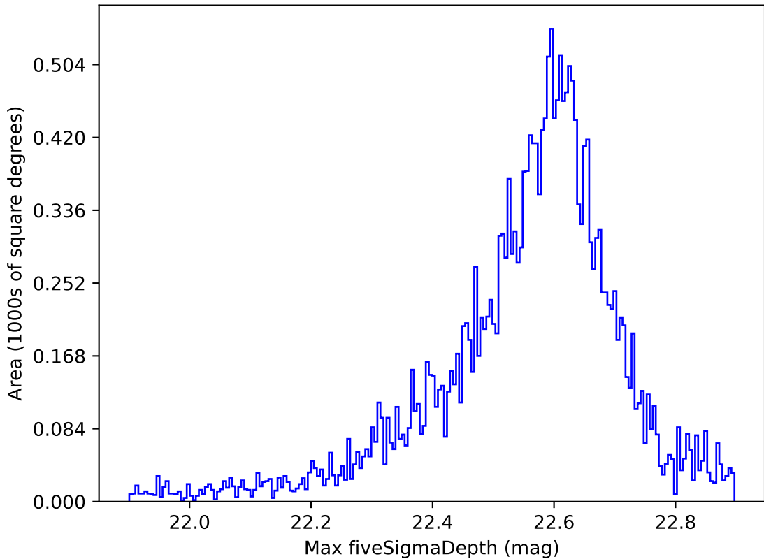
ddf_acor_sf10_ls30_lsr10_v3.4_10yrs All sky y band: Max fiveSigmaDepth
