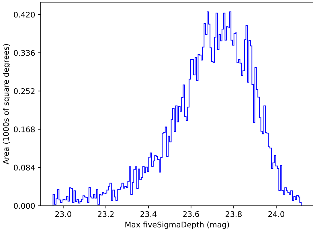
ddf_acor_sf10_ls30_lsr10_v3.4_10yrs All sky u band: Max fiveSigmaDepth
