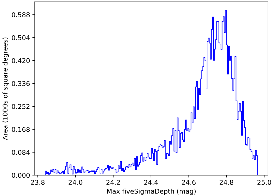
ddf_acor_sf10_lsf30_lsr10_v3.4_10yrs All sky r band: Max fiveSigmaDepth
