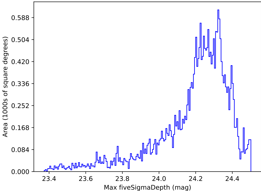
ddf_acor_sf10_lsf30_lsr10_v3.4_10yrs All sky i band: Max fiveSigmaDepth
