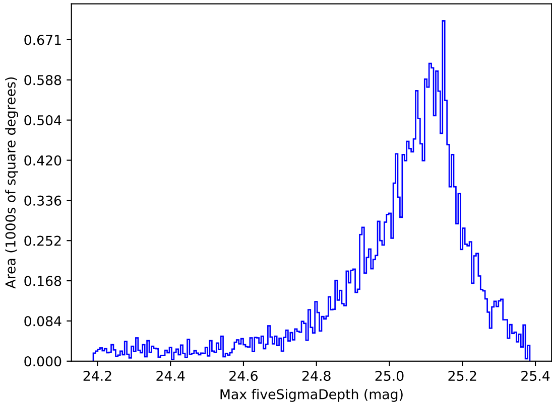
ddf_acor_sf10_lsf30_lsr10_v3.4_10yrs All sky g band: Max fiveSigmaDepth
