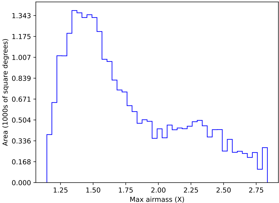
ddf_acor_sf10_lsf30_lsr10_v3.4_10yrs Yr 1 z band: Max airmass
