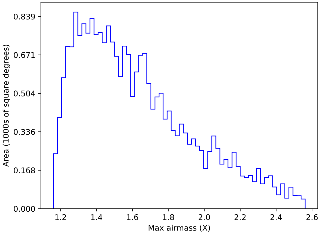
ddf_acor_sf10_lsf30_lsr10_v3.4_10yrs Yr 1 y band: Max airmass
