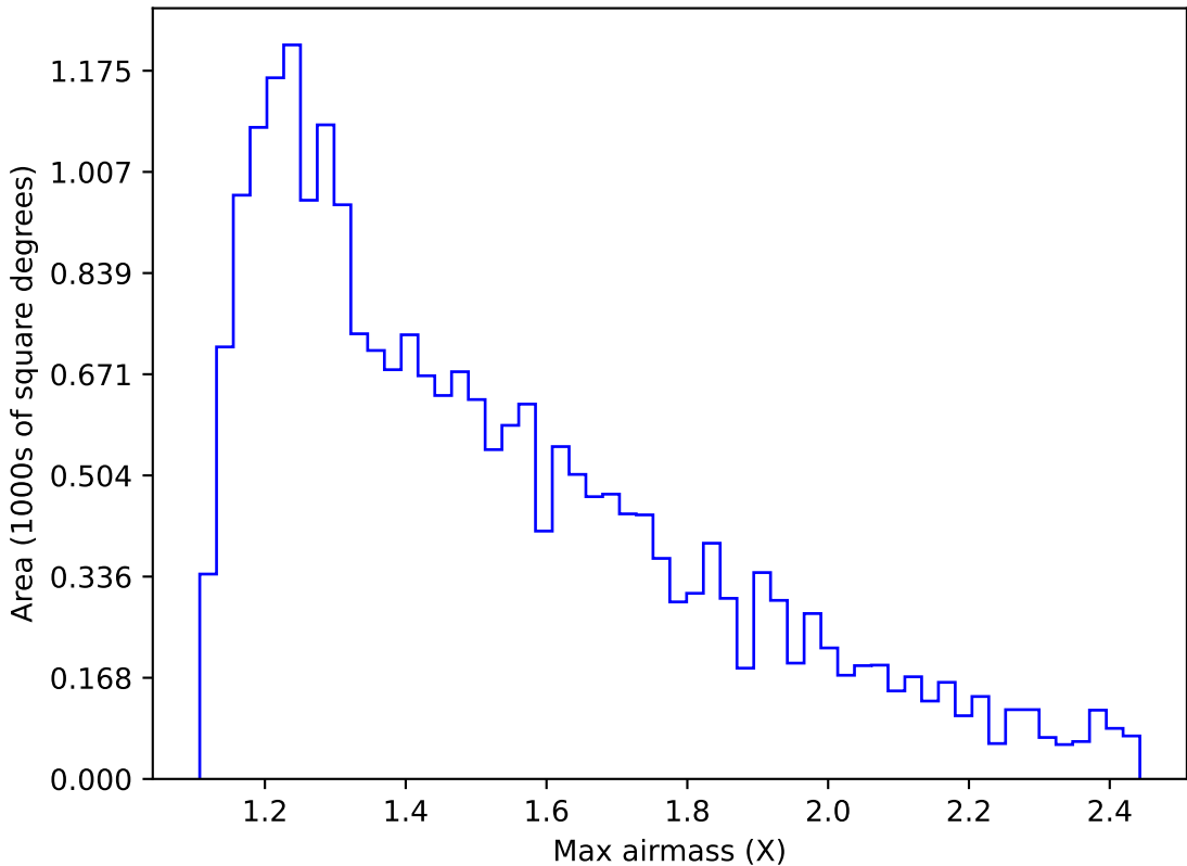
ddf_acor_sf10_lsf30_lsr10_v3.4_10yrs Yr 1 u band: Max airmass
