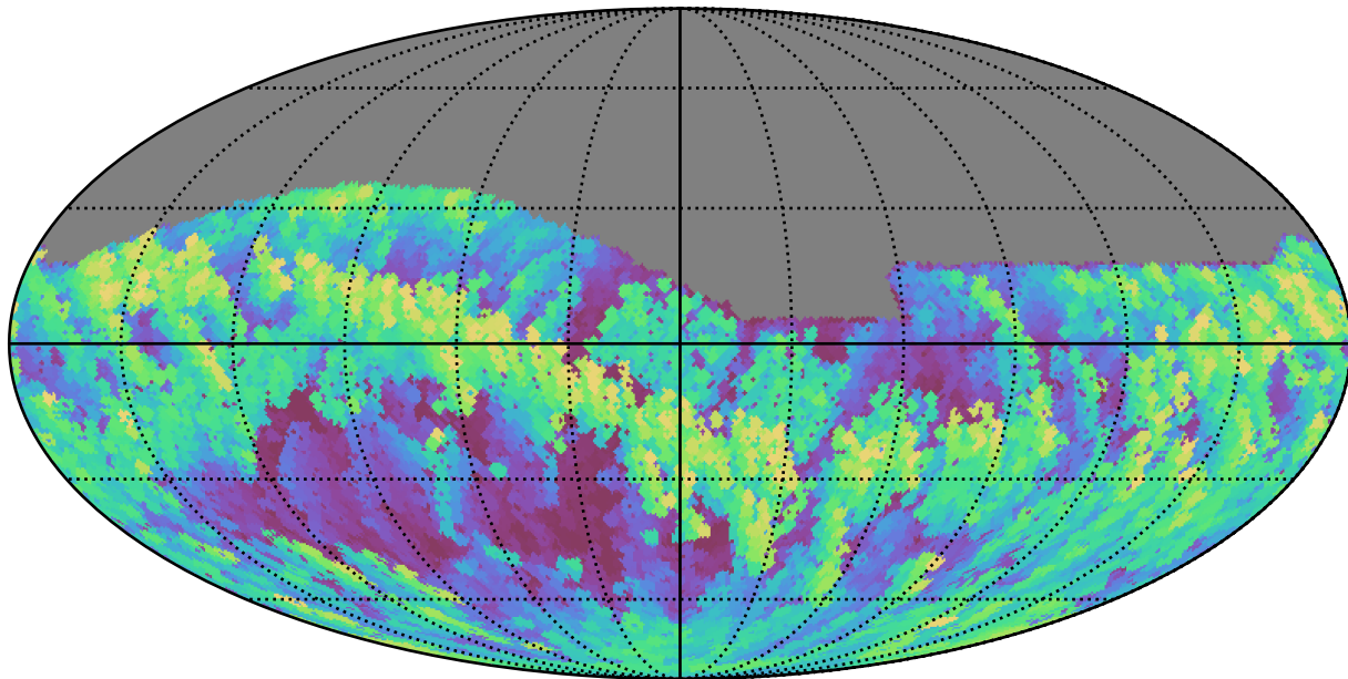
ddf_acor_sf10_lsf30_lsr10_v3.4_10yrs Yr 1 all bands: Max airmass
