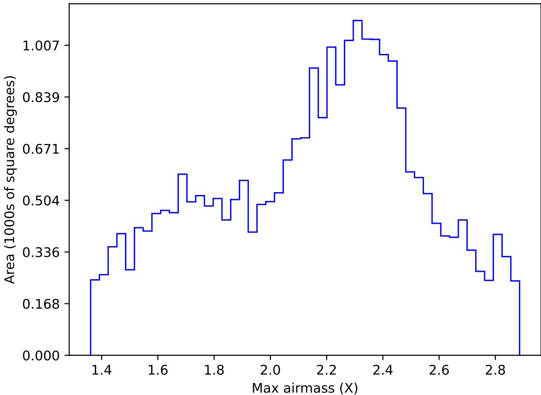
ddf_acor_sf10_lsf30_lsr10_v3.4_10yrs Yr 1 all bands: Max airmass
