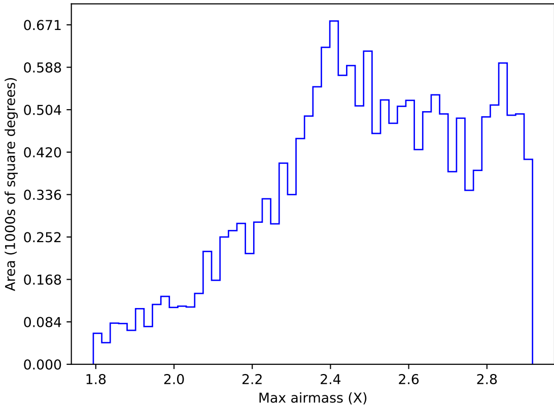
ddf_acor_sf10_lsf30_lsr10_v3.4_10yrs WFD z band: Max airmass
