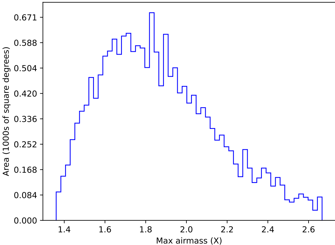
ddf_acor_sf10_ls30_lsr10_v3.4_10yrs WFD u band: Max airmass
