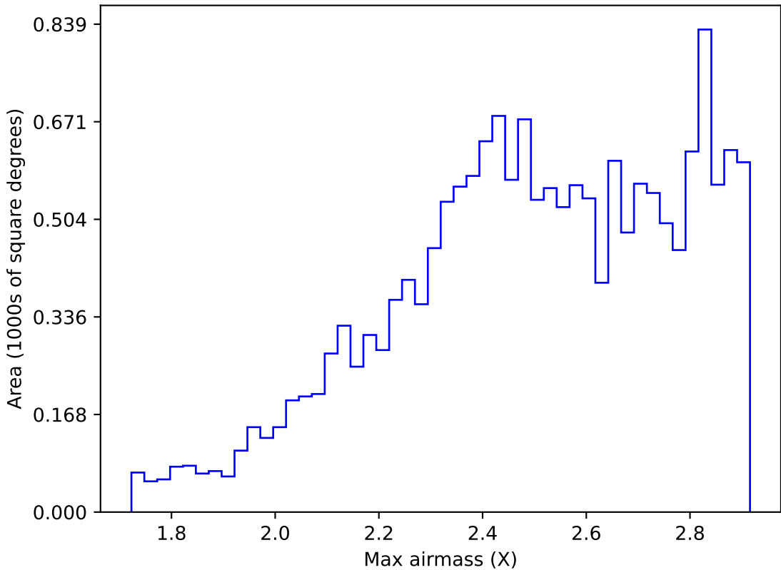
ddf_acor_sf10_lsf30_lsr10_v3.4_10yrs WFD i band: Max airmass
