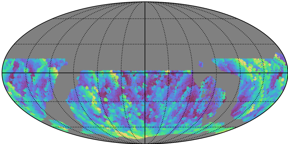
ddf_acor_sf10_lsf30_lsr10_v3.4_10yrs WFD g band: Max airmass
