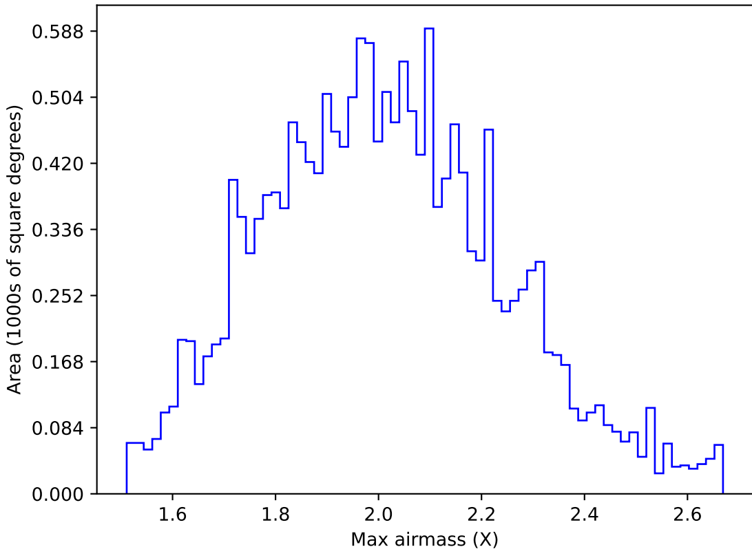
ddf_acor_sf10_lsf30_lsr10_v3.4_10yrs WFD g band: Max airmass
