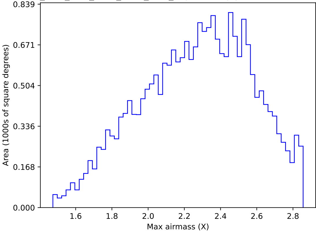
ddf_acor_sf10_lsf30_lsr10_v3.4_10yrs All sky y band: Max airmass
