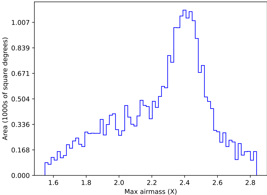
ddf_acor_sf10_lsf30_lsr10_v3.4_10yrs All sky r band: Max airmass
