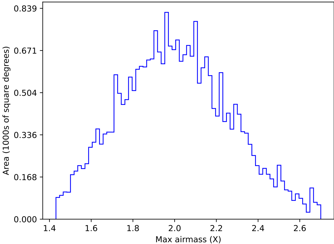
ddf_acor_sf10_lsf30_lsr10_v3.4_10yrs All sky g band: Max airmass
