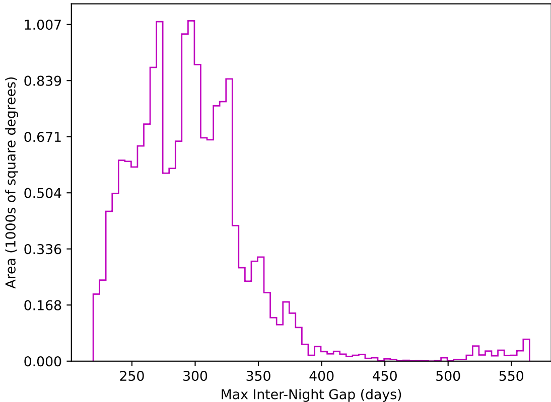
ddf_acor_sf10_lsf30_lsr10_v3.4_10yrs WFD z band: Max Inter-Night Gap
