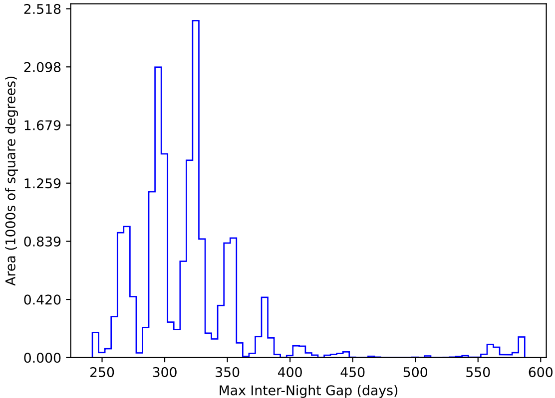
ddf_acor_sf10_lsf30_lsr10_v3.4_10yrs WFD y band: Max Inter-Night Gap
